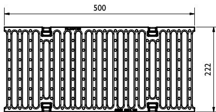
E600kN SW14/200: GJS 17020105
